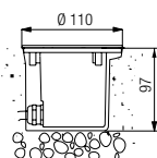
CS4010 (per/for LED 4,5W - LED GU10) Cassaforma in tecnopolimero per vano ad incasso Ø mm 110 - h mm 97 Technopolymer holder to be recessed Ø mm 110 - h mm 97
